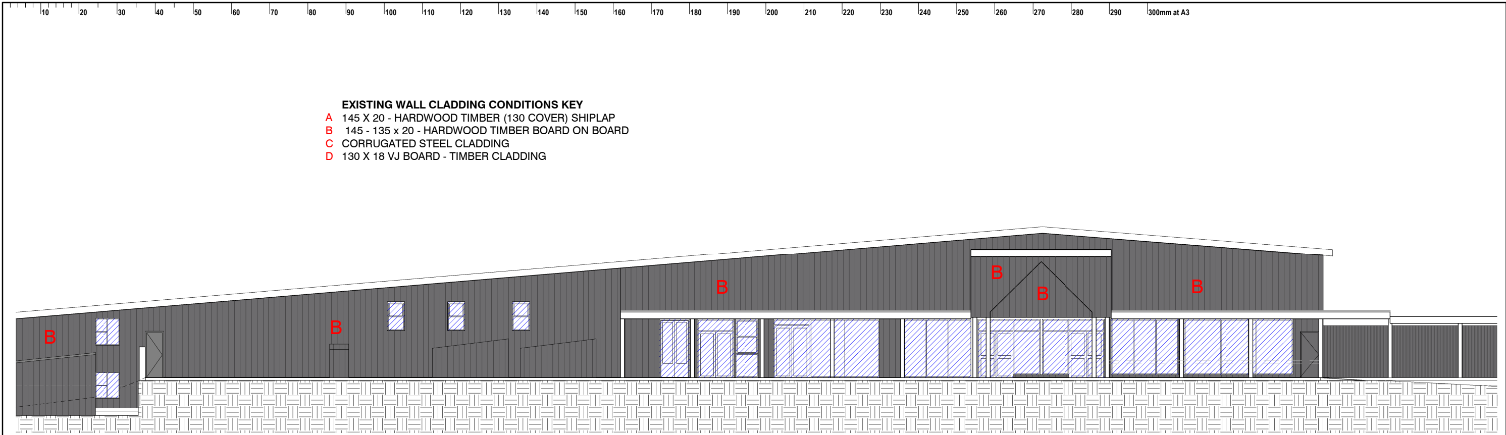
08 ELEVATION - SOUTH - VIEW 2 1 : 200
